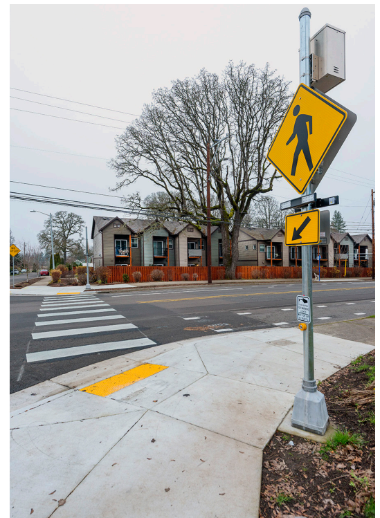
Example of a completed Rectangular Rapid Flashing Beacon (RRFB) crossing on Hall Boulevard at SW Spruce, creating a safer and more visible pedestrian crossing along a busy corridor.
